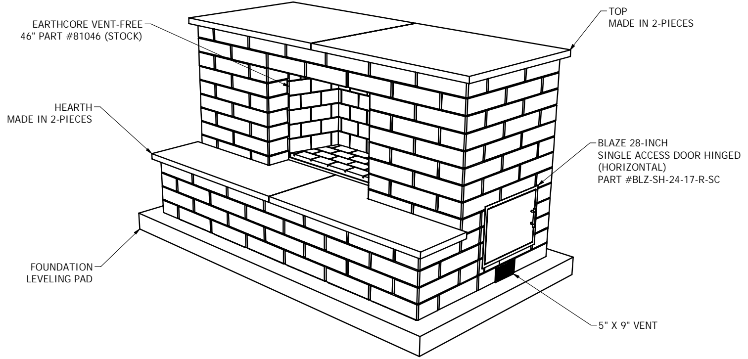
ISOMETRIC VIEW
