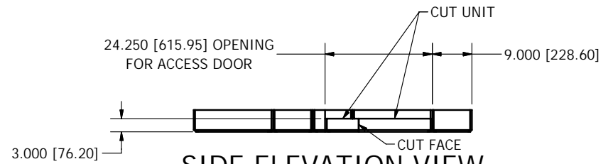
SIDE ELEVATION VIEW
